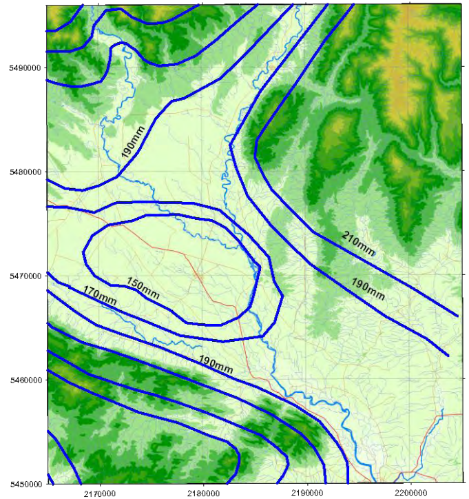
B: Spring isohyets (3-month)
