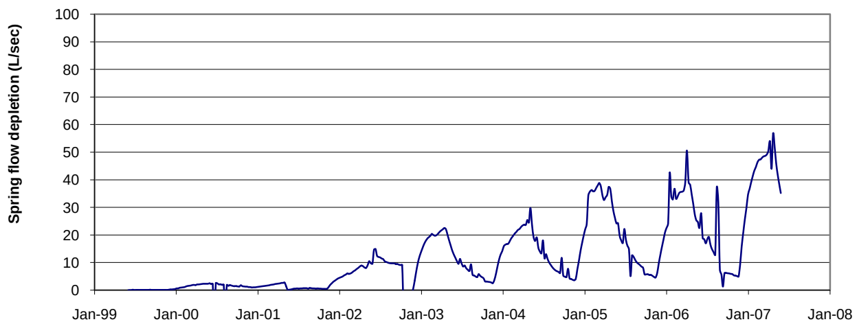
Figure 41: Simulated springflow depletion in Meadow Burn all wells except High/Direct SFD
