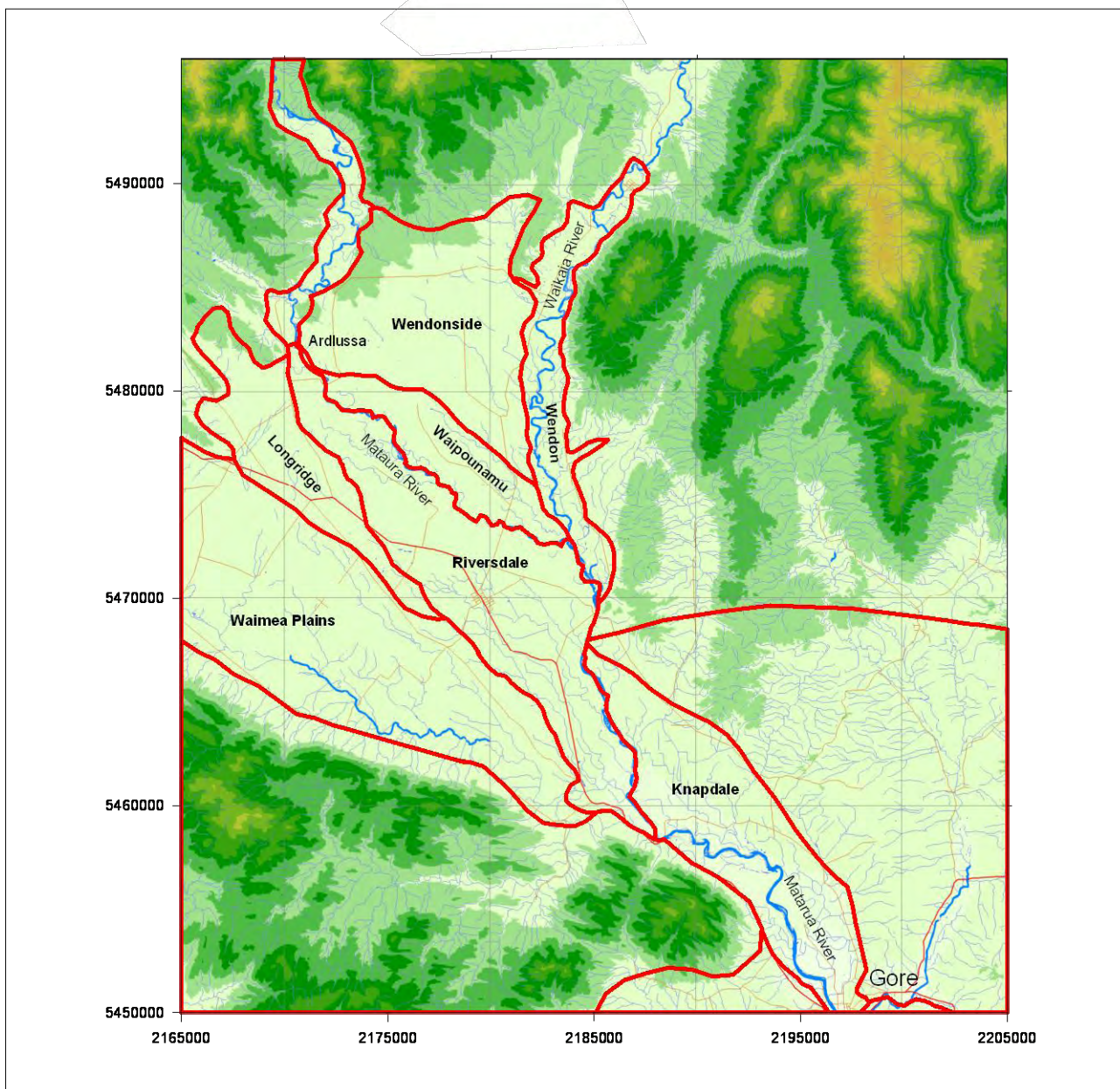
Figure 8: Groundwater management zones
