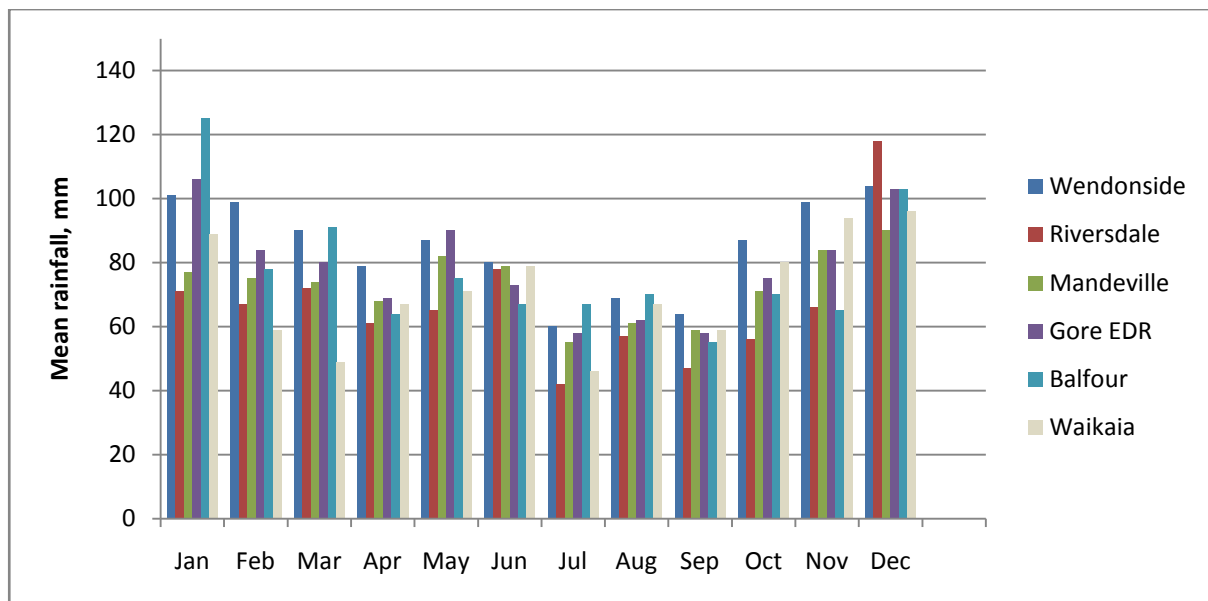
Figure 2: Temporal rainfall patterns relating to rainfall stations
