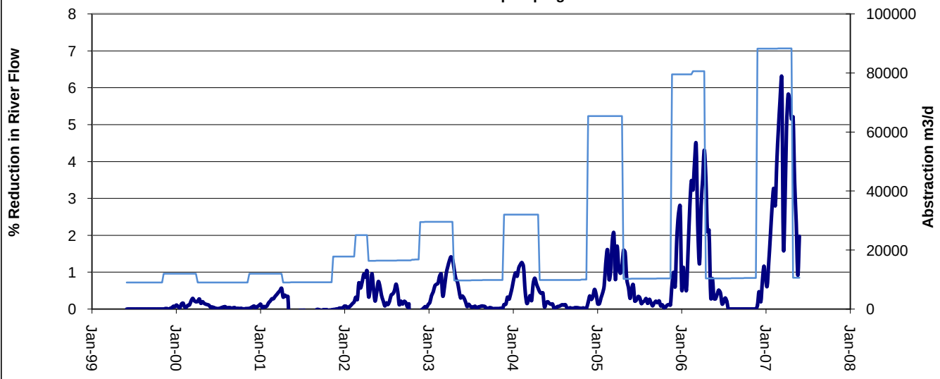
Figure 33: Simulated flow reduction at Riversdale Bridge as percentage of flow in the Maitura River - All wells pumping
