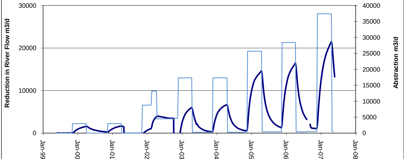
Figure 36: Simulated flow reduction at Pyramid Bridge - all wells except High/Direct SFD
