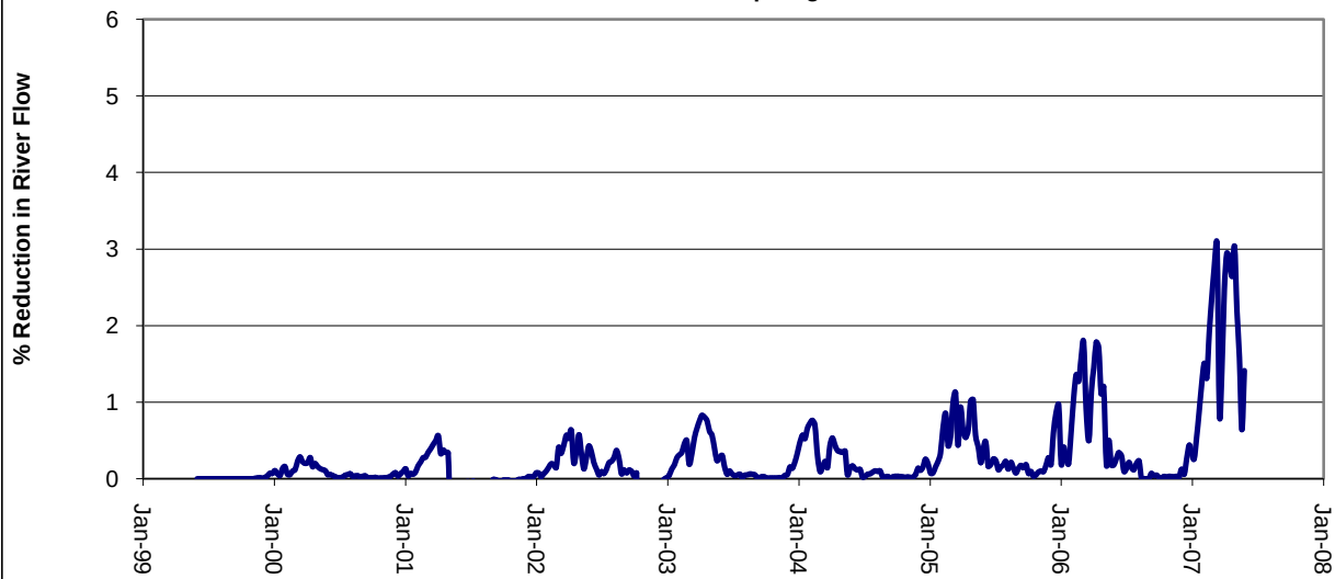
Figure 39: Simulated flow reduction at Riversdale Bridge as percentage of flow in the Mataura River - all wells except High/Direct SFD
