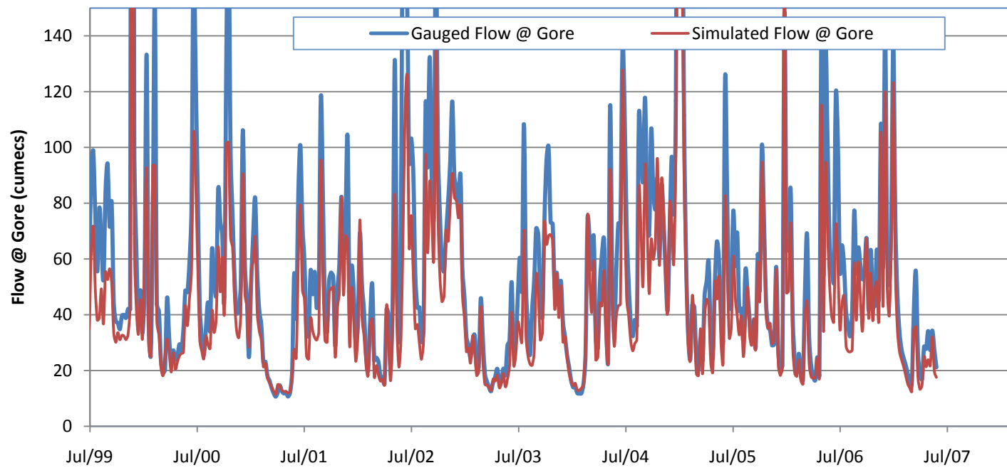
Figure 29: Simulated vs Gauged Flow in the Mataura River @ Gore
