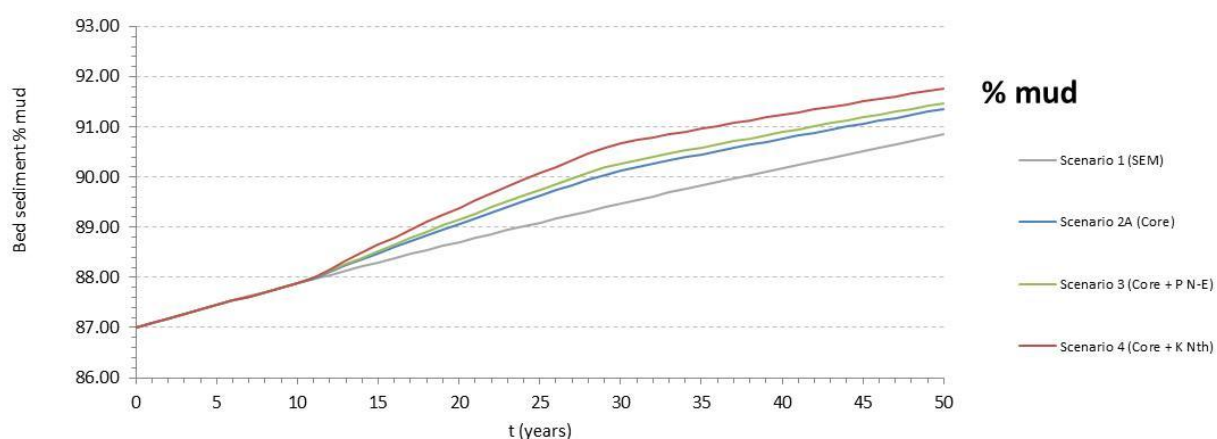
Figure 4-18 Predicted change in the mud content of estuary bed-sediments under Scenarios 1, 2A, 3 and 4, ERU7 (Glassons Creek Inner)
