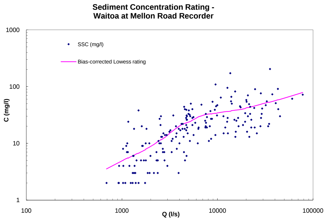
Figure A-5: Waitoa at Mellon Road sediment concentration rating.
