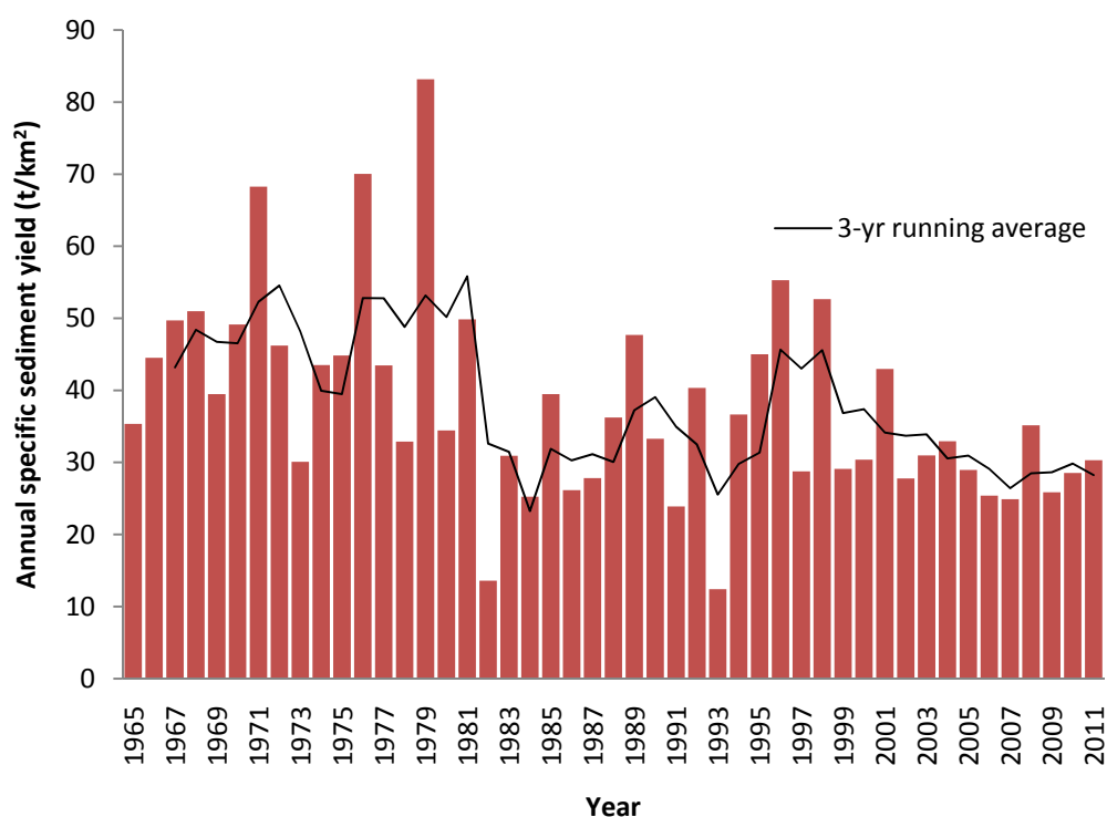
Figure 3-2: Specific annual sediment yields and three year running average yield between 1965 and 2011 at Waihou at Te Aroha Bridge.
