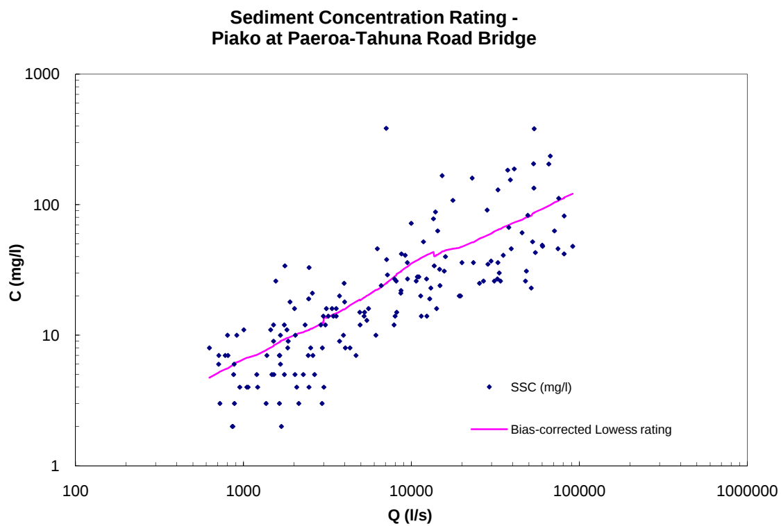
Figure A-12: Piako at Paeroa-Tahuna Road Bridge sediment concentration rating.
