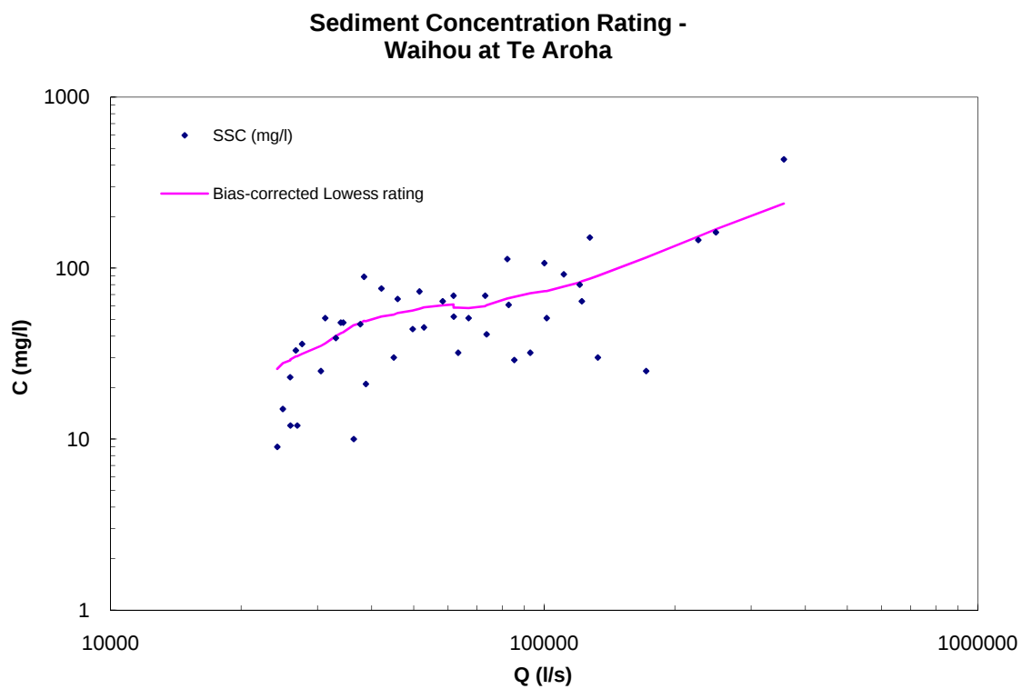
Figure A-16: Waihou at Te Aroha sediment concentration rating.
