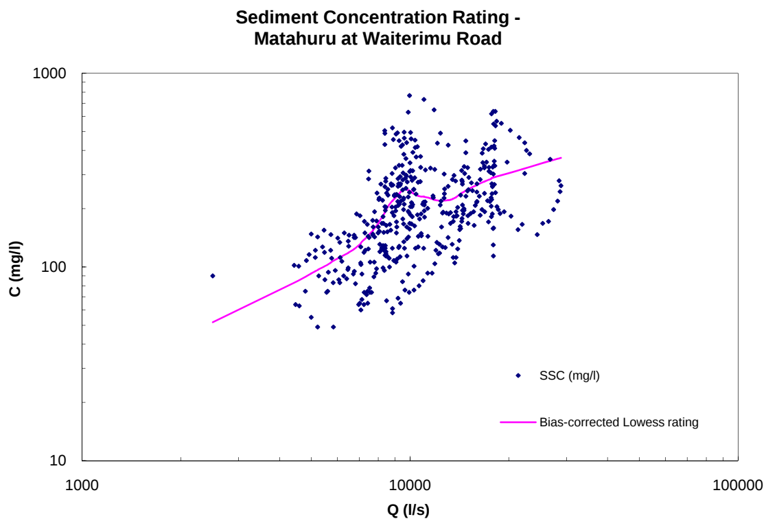
Figure A-19: Matahuru at Waiterimu Road sediment concentration rating.
