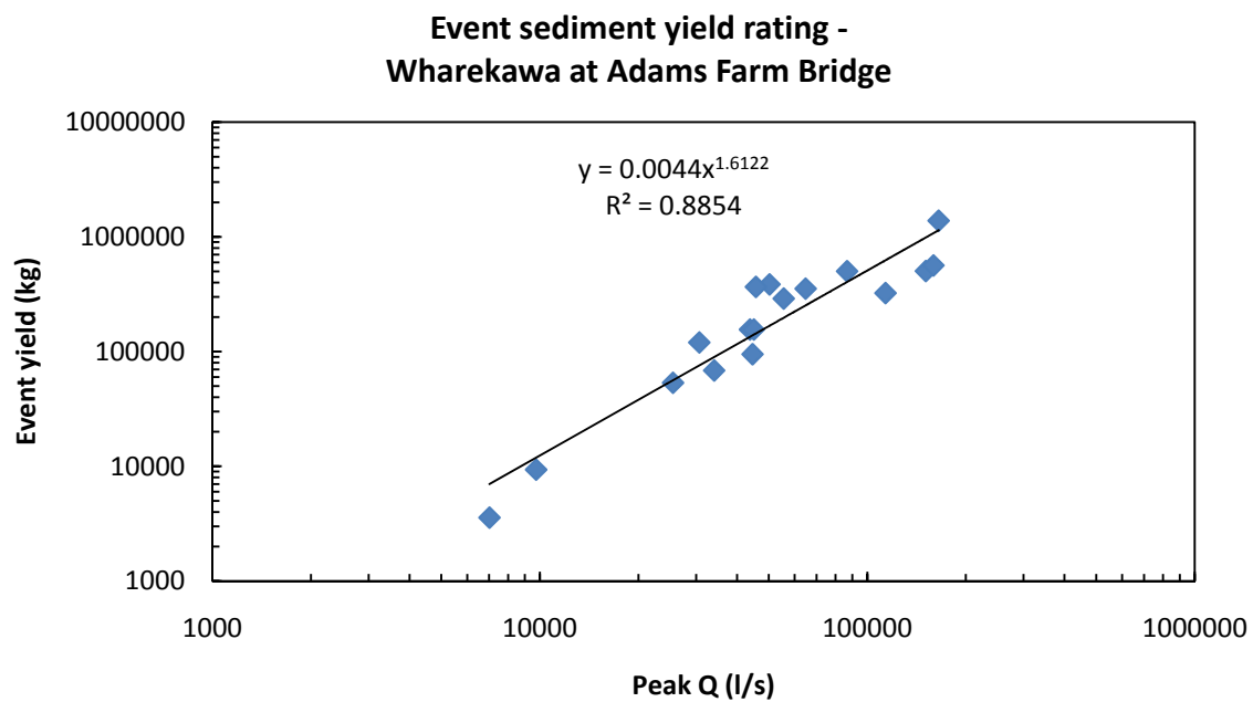
Figure B-7: Wharekawa at Adams Farm Bridge event yield rating. This rating has a power relationship.
