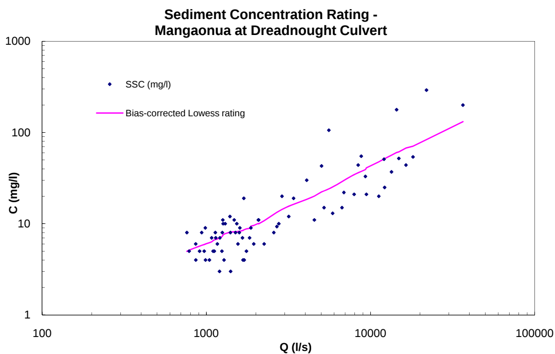
Figure A-1: Mangaonua at Dreadnought Culvert SH1 sediment concentration rating.
