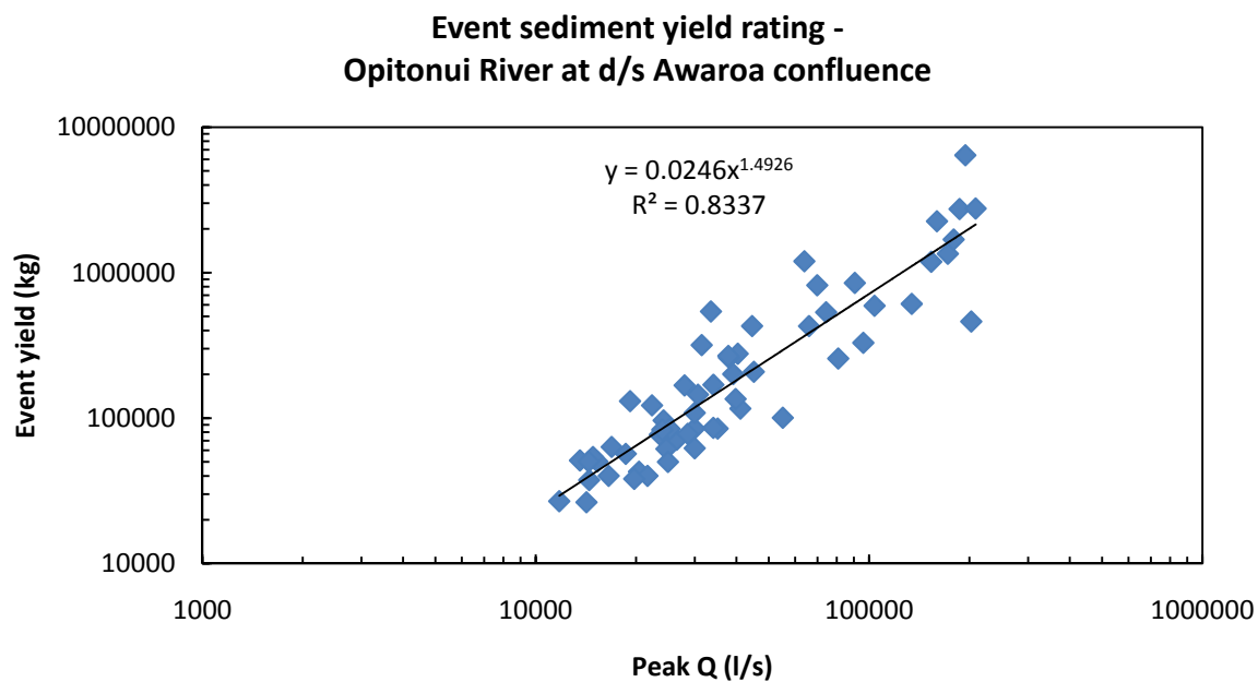
Figure B-3: Opitonui River at d/s Awaroa confluence event yield rating. This rating has a power relationship.
