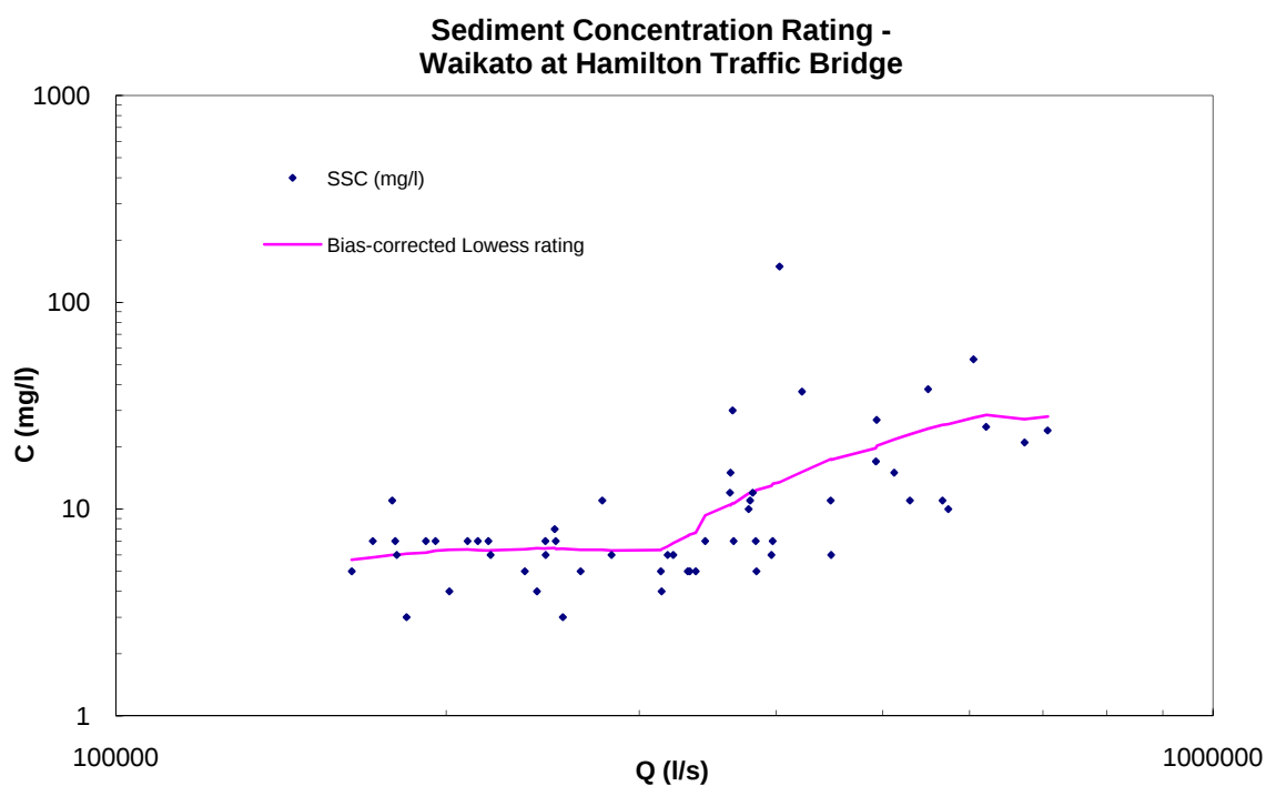
Figure A-2: Waikato at Hamilton Traffic Bridge sediment concentration rating.
