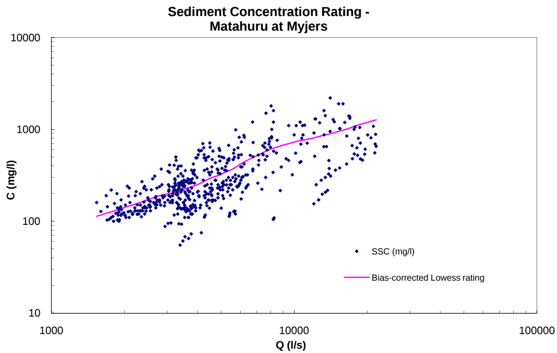
Figure A-6: Matahuru at Myers sediment concentration rating.
