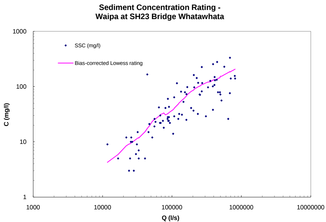
Figure A-23: Waipa at SH23 Bridge Whatawhata sediment concentration rating.
