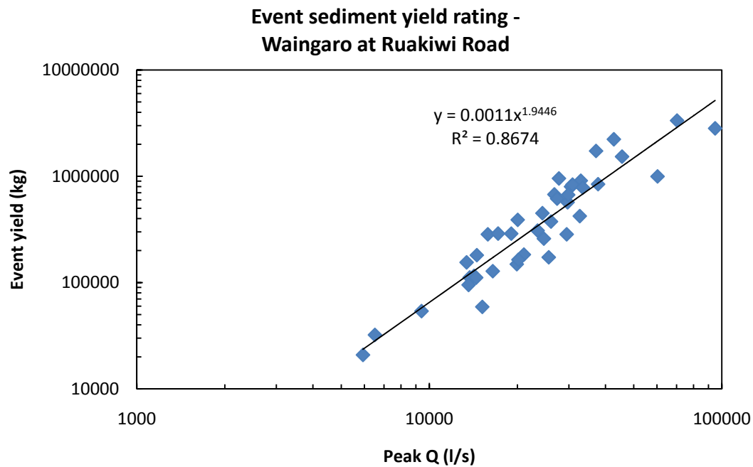
Figure B-5: Waingaro at Ruakiwi Road event yield rating. This rating has a power relationship.
