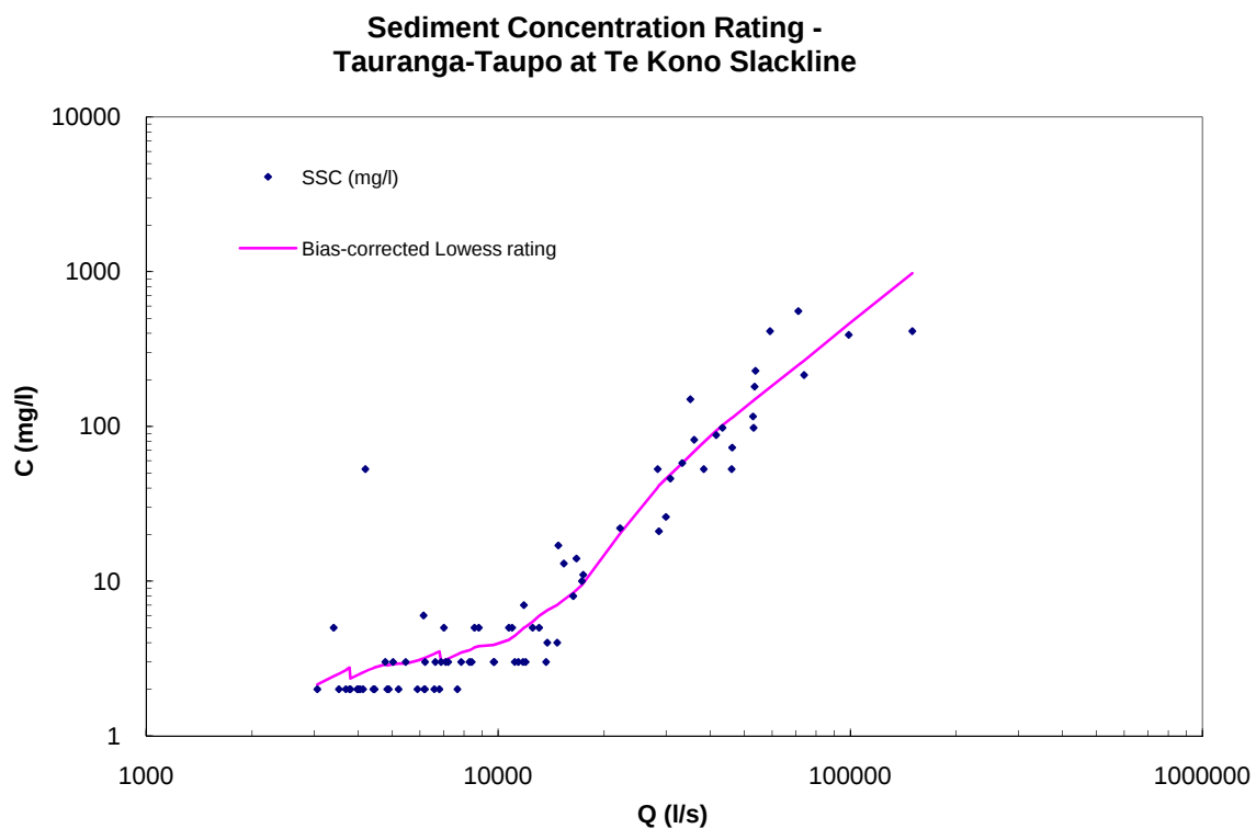
Figure A-15: Tauranga-Taupo at Te Kono Slackline sediment concentration rating.
