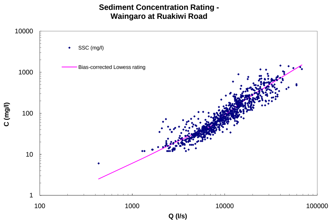
Figure A-18: Waingaro at Ruakiwi Road sediment concentration rating.
