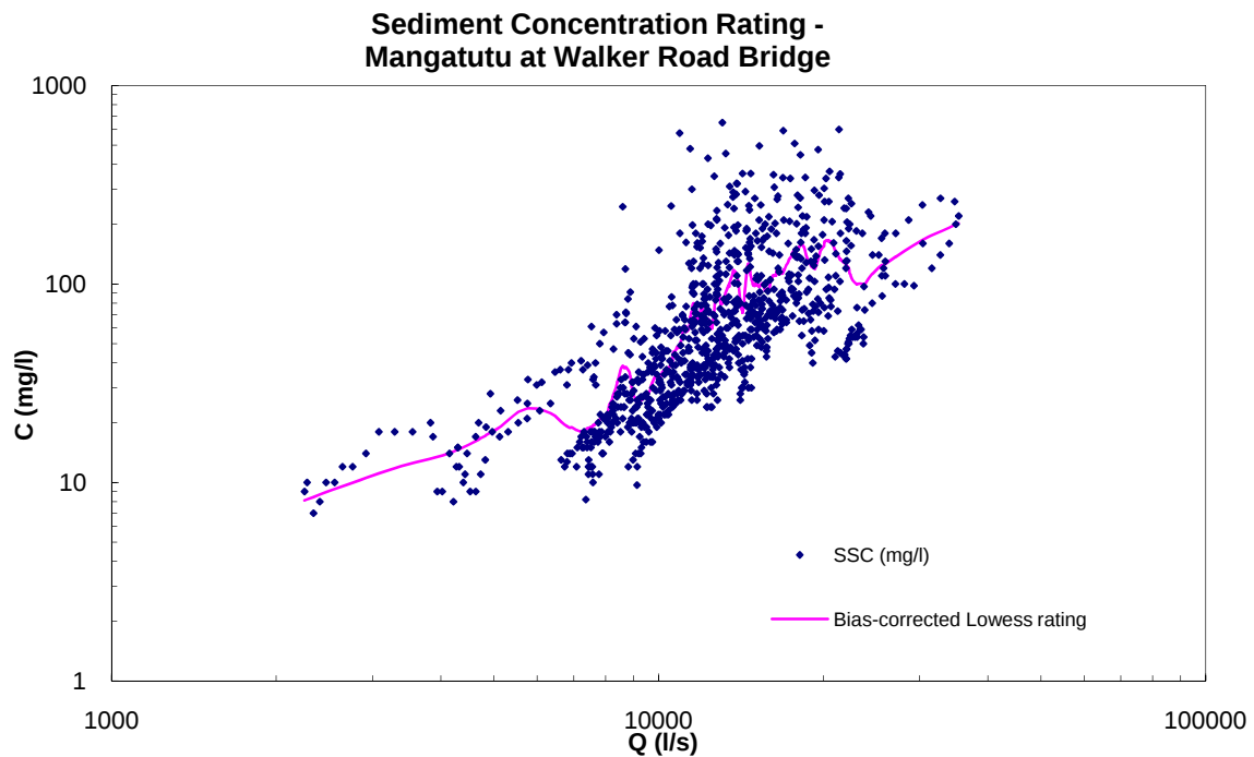
Figure A-4: Mangatutu at Walker Road Bridge sediment concentration rating.
