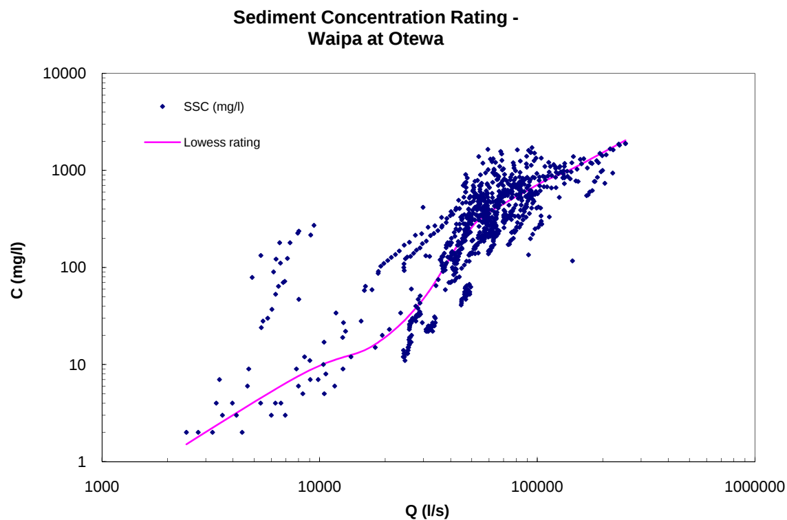
Figure A-9: Waipa at Otewa sediment concentration rating.
