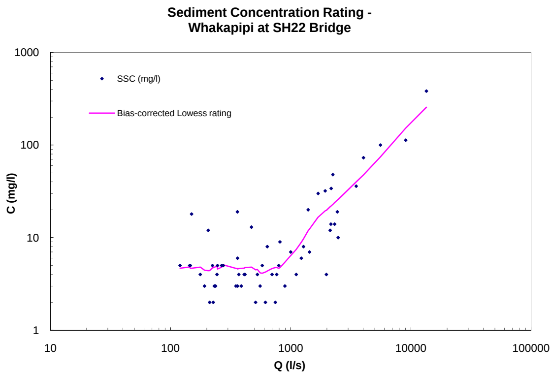
Figure A-21: Whakapipi at SH22 Bridge sediment concentration rating.
