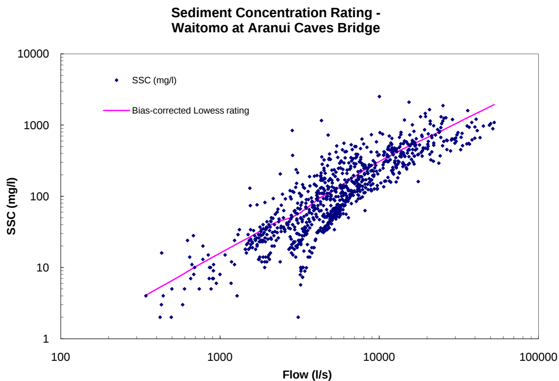
Figure A-20: Waitomo at Aranui Caves Bridge sediment concentration rating.
