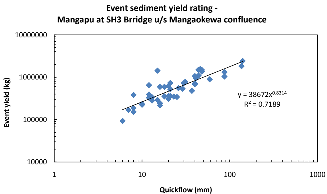
Figure B-8: Mangapu at SH3 Bridge u/s Mangaokewa confluence event yield rating. This rating has a power relationship.
