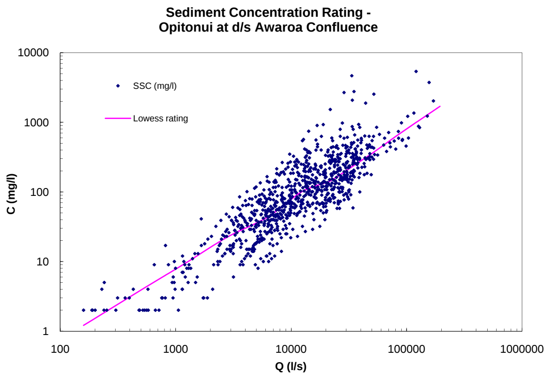
Figure A-8: Opitonui at d/s Awaroa confluence sediment concentration rating.
