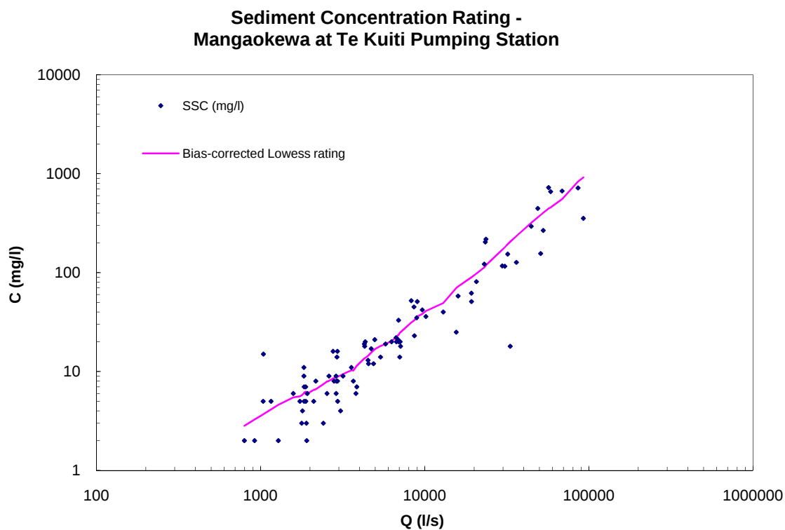
Figure A-17: Mangaokewa at Te Kuiti Pumping Station sediment concentration rating.
