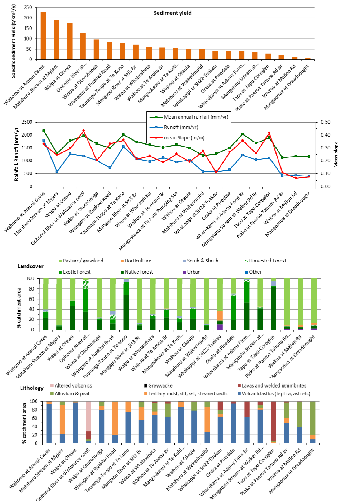
Figure 3-1: Specific sediment yield vs. catchment characteristics. Includes catchment mean annual rainfall and runoff, mean slope, and % area by land-cover and lithology. Sites are ordered (left to right) by decreasing sediment yield.
