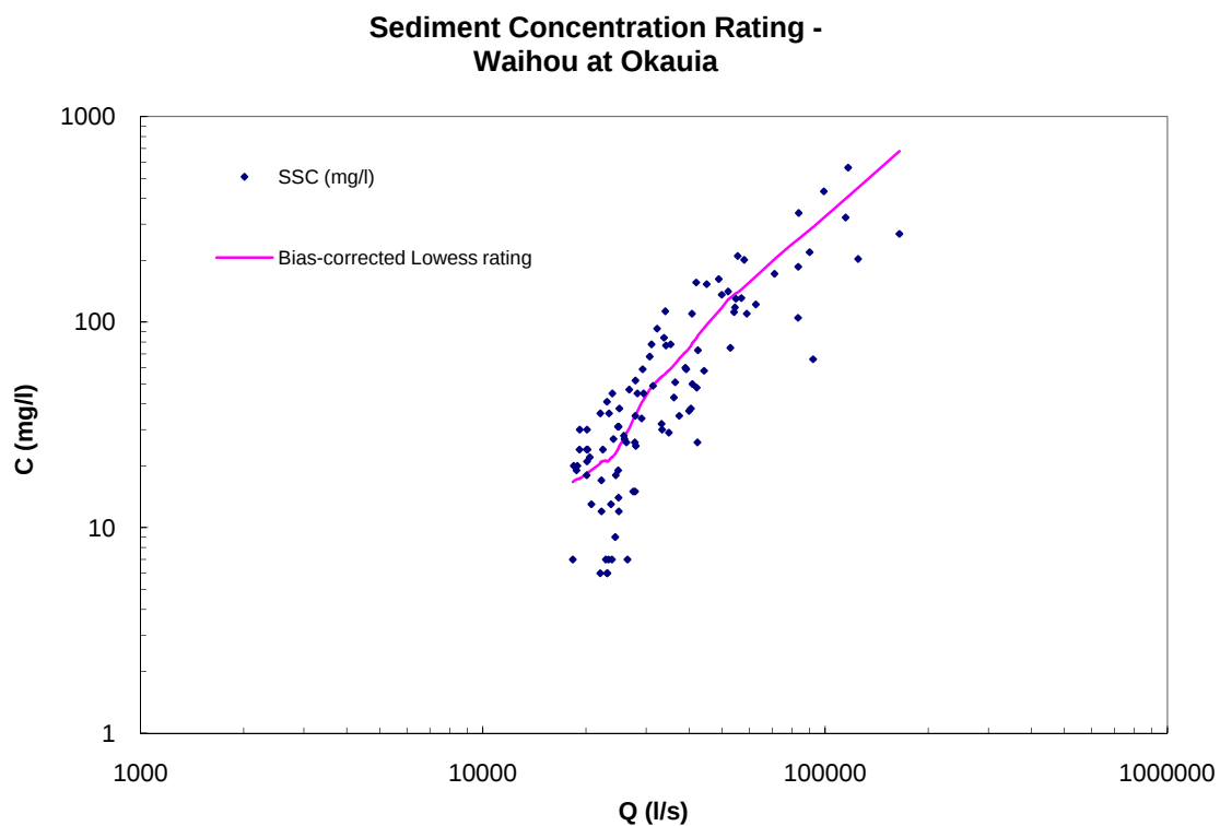
Figure A-7: Waihou at Okauia sediment concentration rating.
