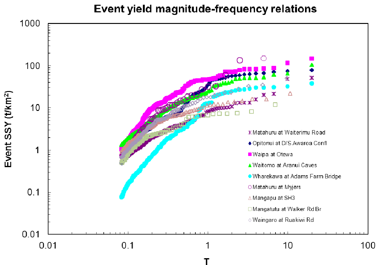
Figure 3-3: Event-yield magnitude-frequency relations for auto-sampled sites. Return period, T , in years.
