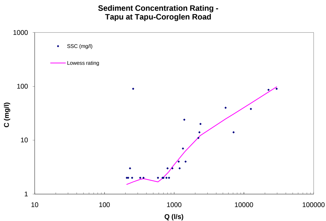
Figure A-14: Tapu at Tapu-Coroglen Road sediment concentration rating.
