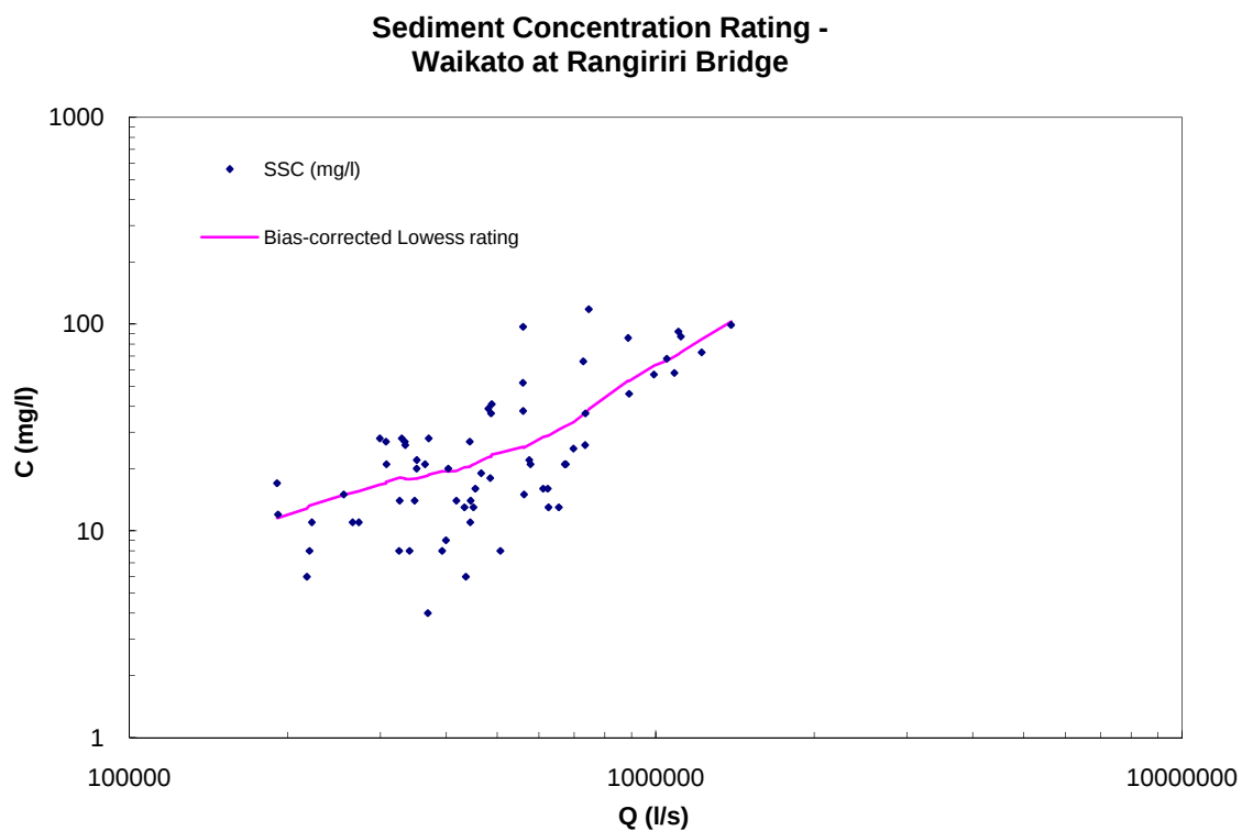
Figure A-13: Waikato at Rangiriri Bridge sediment concentration rating.
