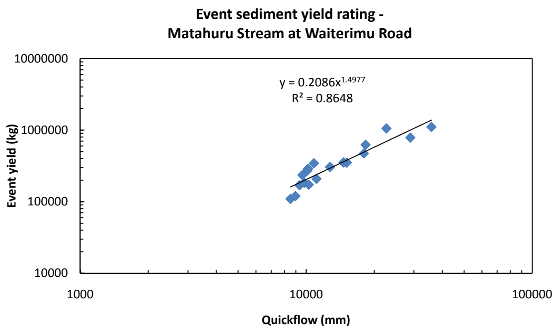
Figure B-1: Matahuru Stream at Waiterimu Road event yield rating. This rating has a power relationship.
