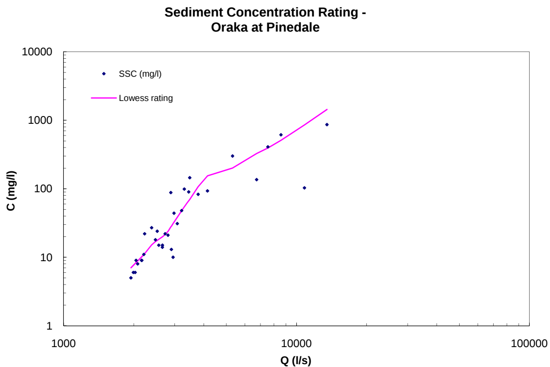
Figure A-11: Oraka at Pinedale sediment concentration rating.
