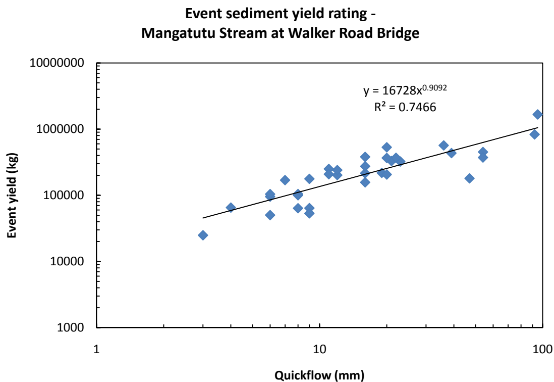
Figure B-2: Mangatutu at Walker Road Bridge event yield rating. This rating has a power relationship.
