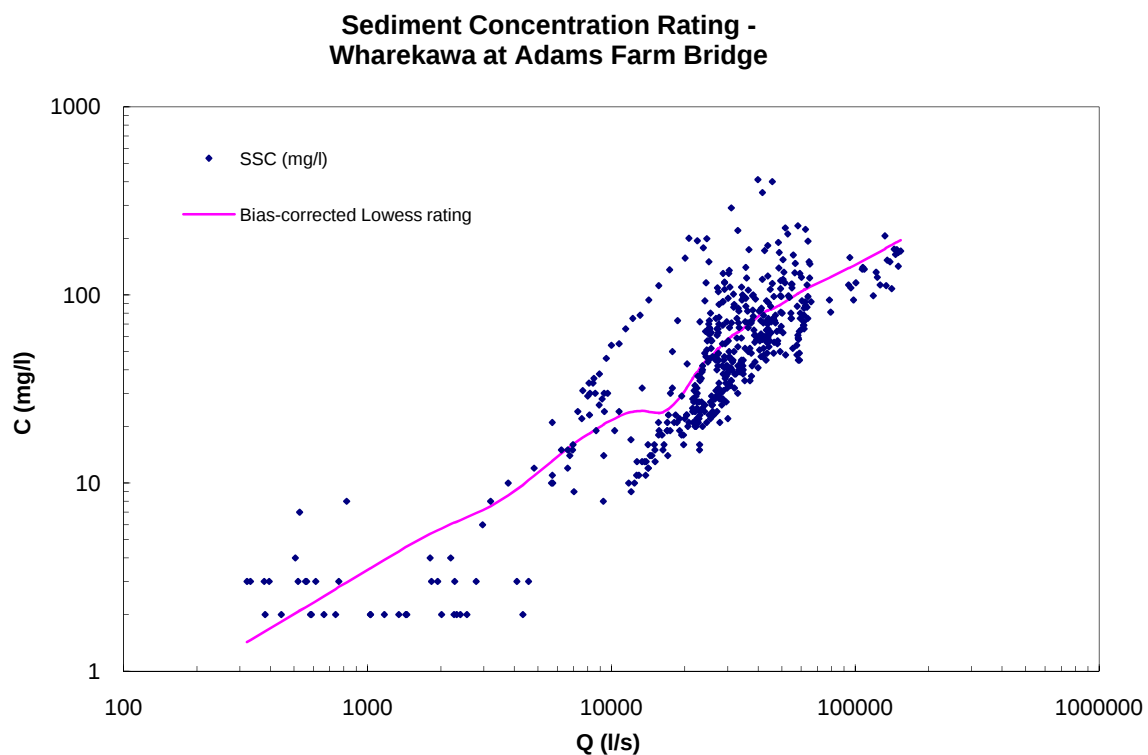
Figure A-22: Wharekawa at Adams Farm Bridge sediment concentration rating.
