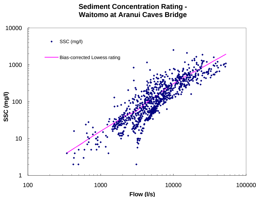
Figure 2-1: Example of a suspended sediment concentration rating from Waitomo at Aranui Caves Bridge catchment. The rating function is a bias-corrected LOWESS fit.
