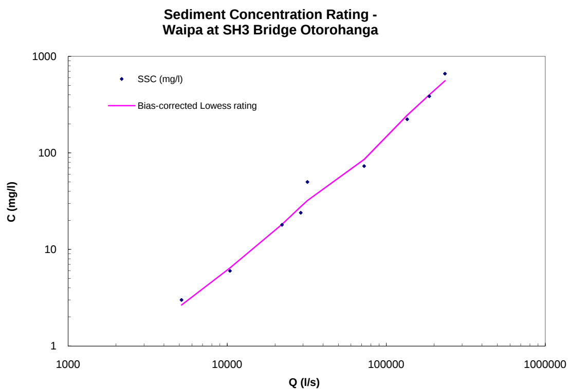
Figure A-10: Waipa at SH3 Bridge Otorohanga sediment concentration rating.
