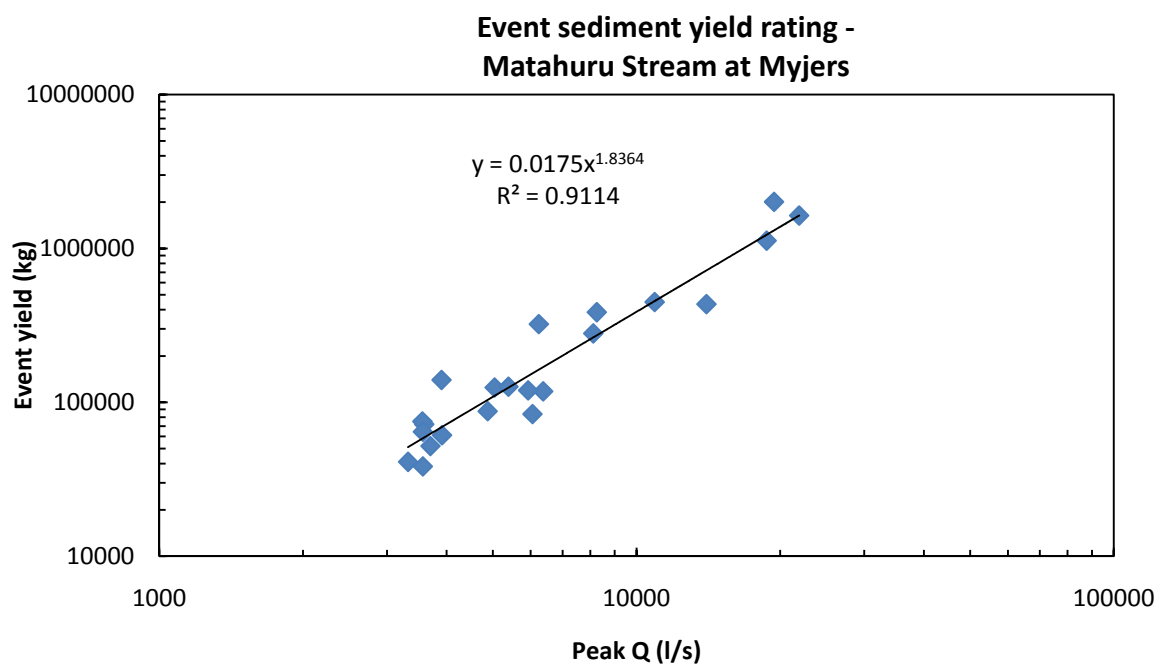
Figure B-9: Matahuru Stream at Myjers event yield rating. This rating has a power relationship.
