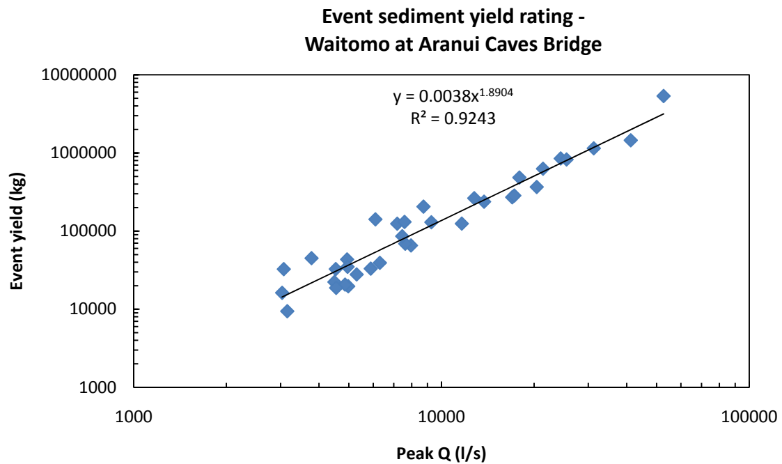
Figure B-6: Waitomo at Aranui Caves event yield rating. This rating has a power relationship.
