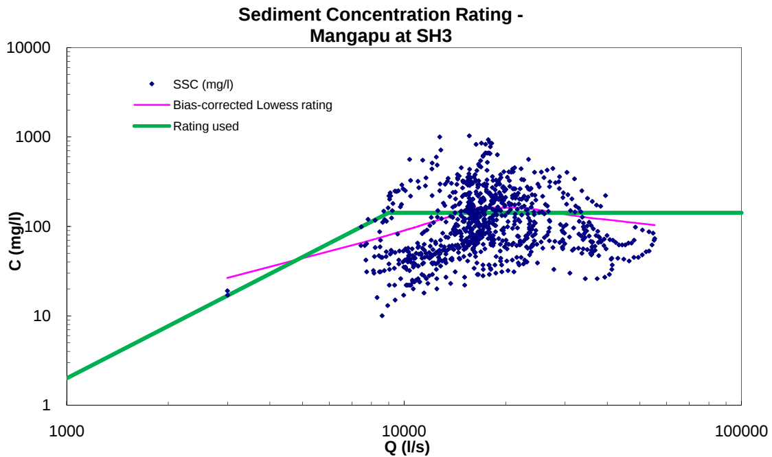
Figure A-3: Mangapu at SH3 sediment concentration rating. NB Due to the broad scatter of data at this site, the lowess rating was not considered appropriate. Instead, a simple rating was developed, using the mean SSC for Q > 9000 l/s and, for Q < 9000 l/s SSC tends to 0 mg/l as flow tends to 0 l/s.
