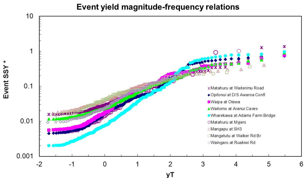
Figure 3-4: Normalised event-yield magnitude-frequency relations for auto-sampled sites. Event specific sediment yield (SSY) has been normalised by the mean annual specific sediment yield. The return period is represented by the extreme value reduced variate, yT .
