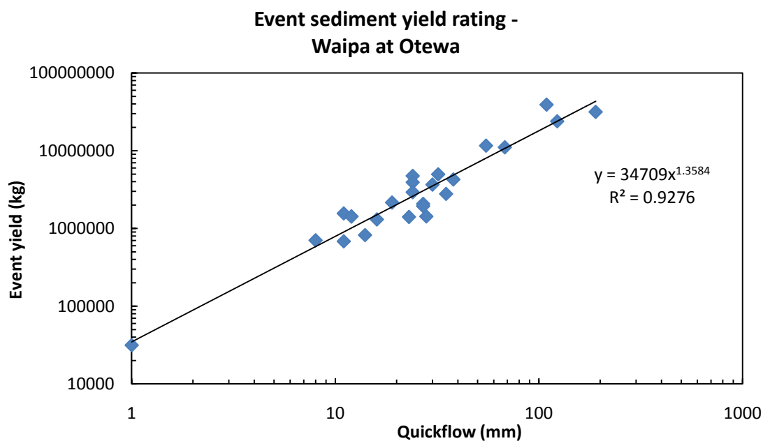
Figure B-4: Waipa at Otewa event yield rating. This rating has a power relationship.
