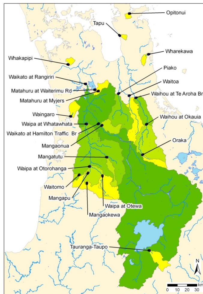
Figure 1-1: Study catchment locations within the Waikato region.
