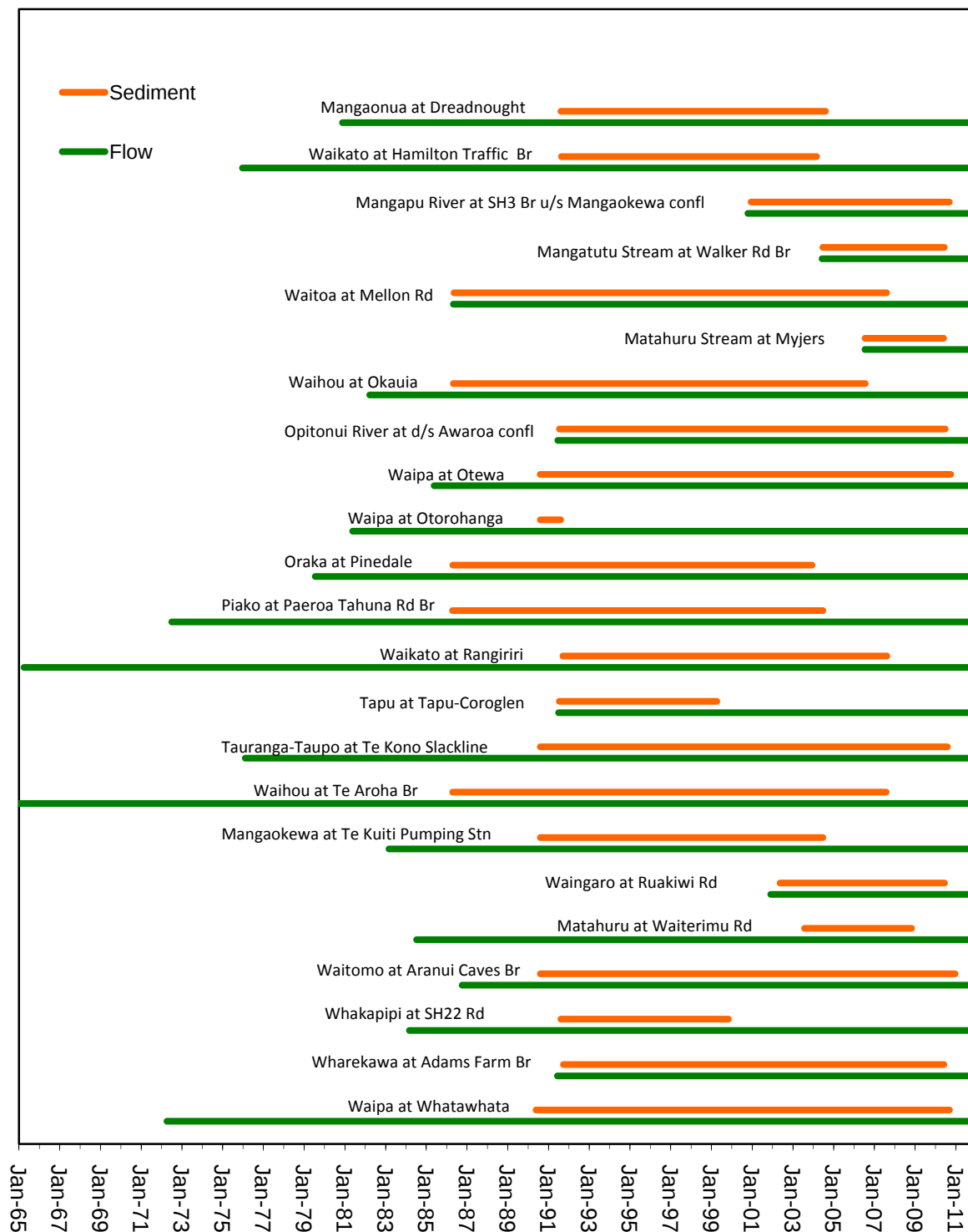
Figure 1-2: Periods of time over which sediment concentration and flow data are available for each catchment.
