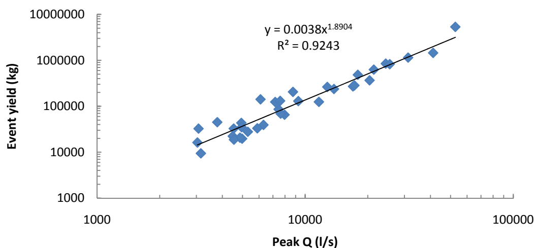
Figure 2-2: Example of an event yield rating from Waitomo at Aranui Caves Bridge catchment. This rating has a power relationship.
