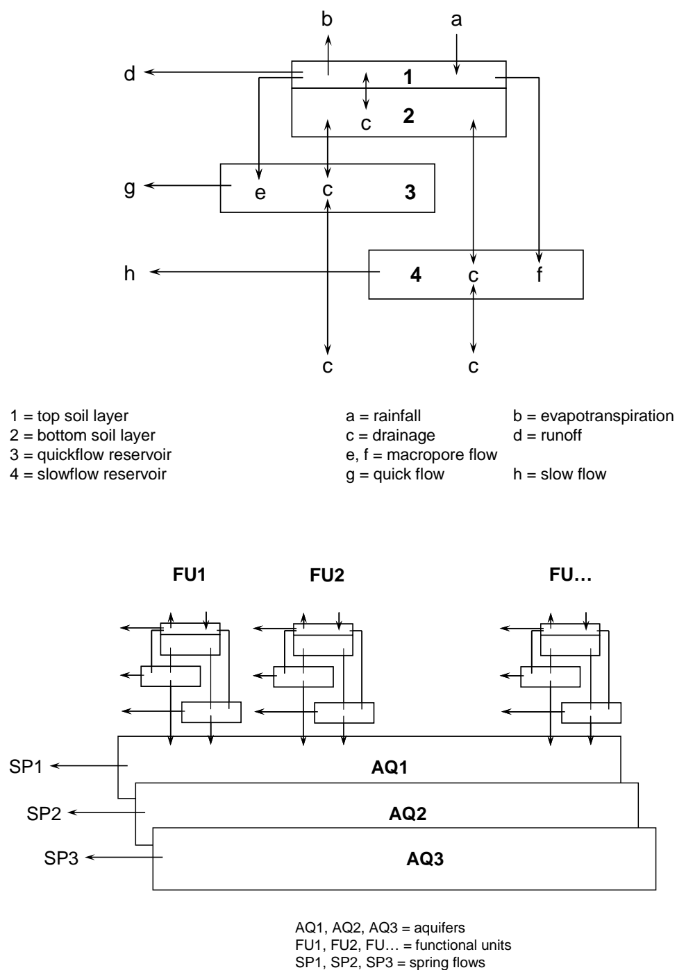
Figure 3: Conceptual rainfall-runoff model that operates in each Functional Unit (top) and connections between Functional Units, Aquifers and Springs (bottom).
